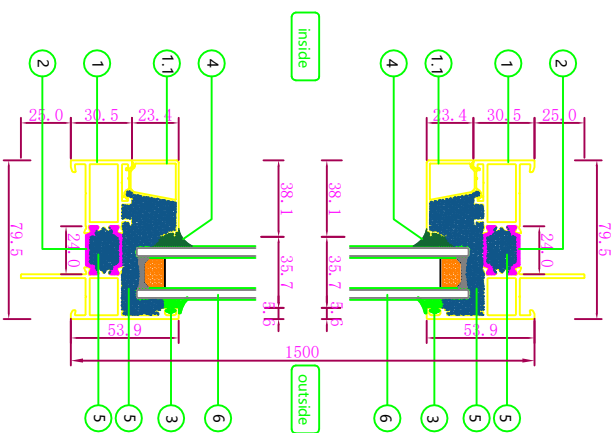
B-B profile
